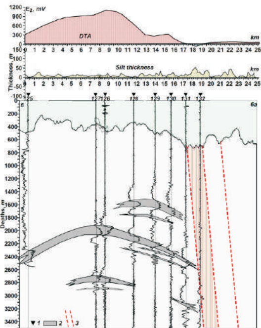
Fig. 6. Interpreted geoelectrical cross-section of the crust of the “hydrocarbon deposit” type in Palmer Deep area. Legend: 1 – VERS-points 125-132; 2 – anomalous polarized layers of “hydrocarbon deposit” type; 3 – tectonic fracture zone.
