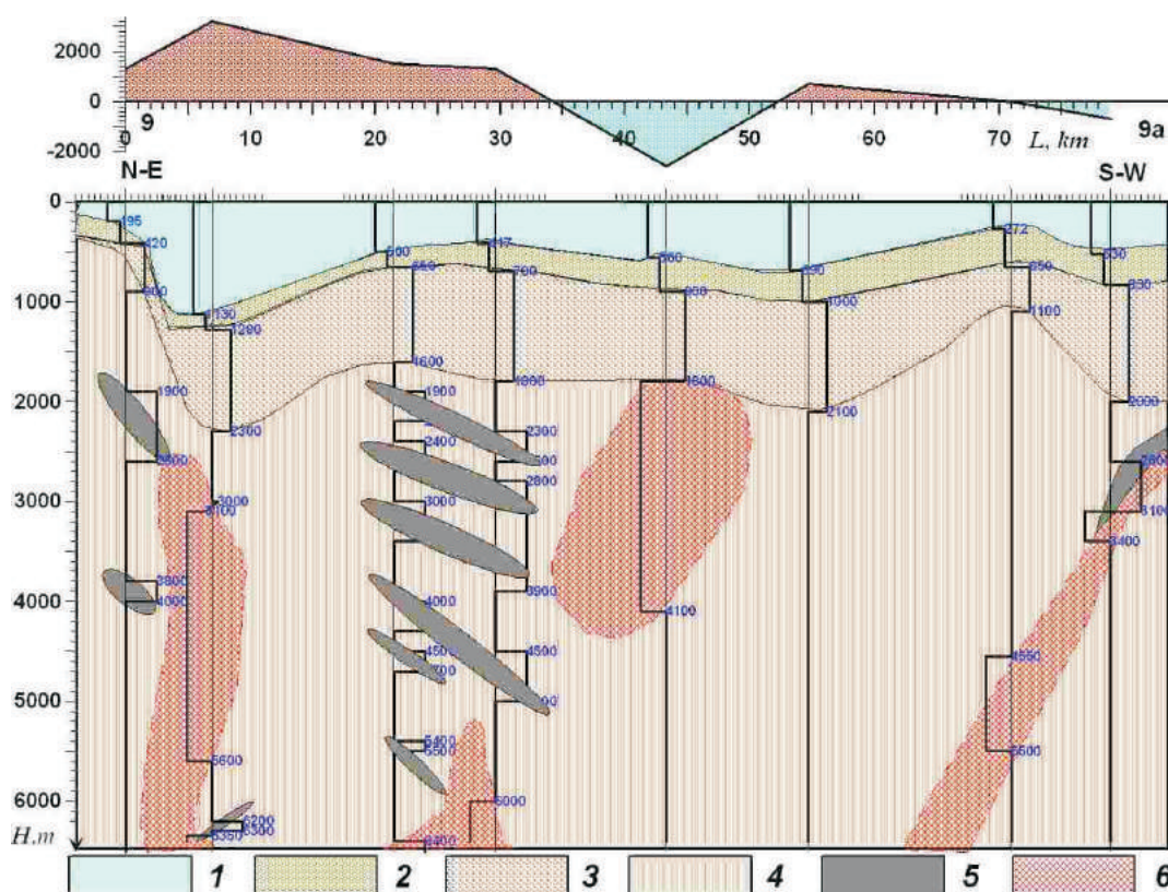
Fig. 4. Interpreted geoelectrical cross-section of the upper part of the crust along the profile 9-9a. Location of profile is shown on Fig.1 (A,B). Legend is shown on Fig. 3.
