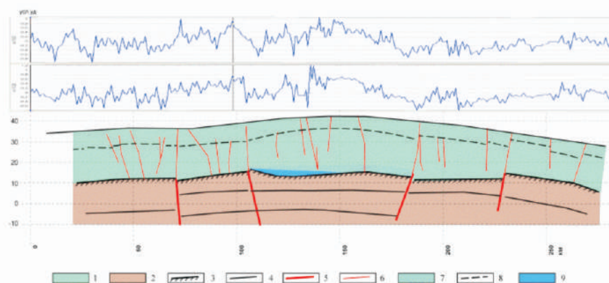
Fig.5. Geology-geophysical section through central glacier part by A'-A profile (data of 2007) with the wavelet components of the signal (above).
