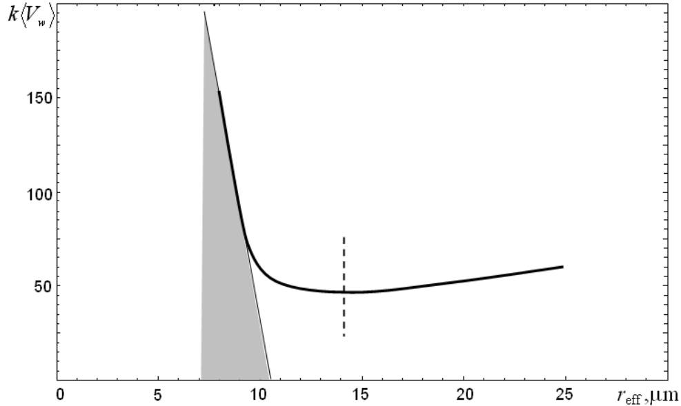
Fig. 4. Mean total volume of liquid water \langle V_w \rangle in the atmosphere as a function of cloud droplet effective radius (CDR). Minimum at r_{\text{eff}} \approx 14 \mu\text{k} (vertical dotted line) corresponds to the so-called precipitation threshold. Left-hand part with respect to the minimum (hatched) is defined by the inverse linear dependence \langle V_w \rangle from CDR.
